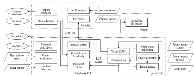
Fig. 3. Overall system architecture
