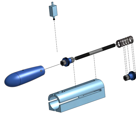
Fig. 2. Exploded-view model of torpedo in launcher
